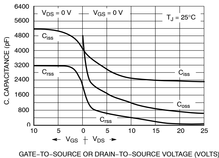
Figure 7. Capacitance Variation
